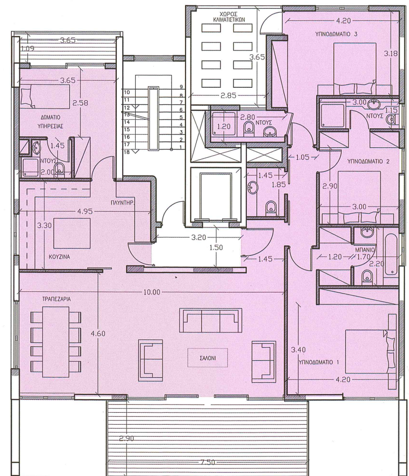
Fifth - Ninth Floor Plan
